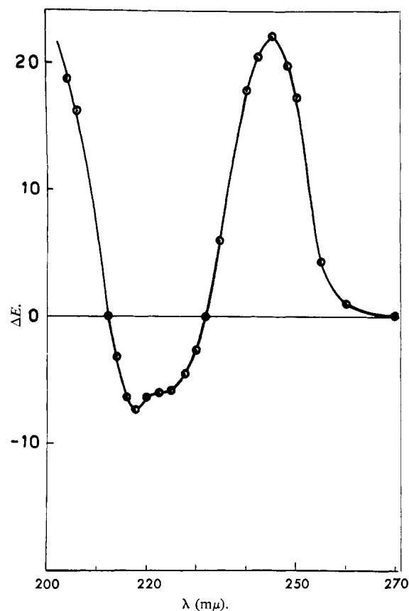
FIGURE 2: Circular dichroism of poly- N ω -carbobenzoxy- L - p -aminophenylalanine in tetrahydrofuran.
