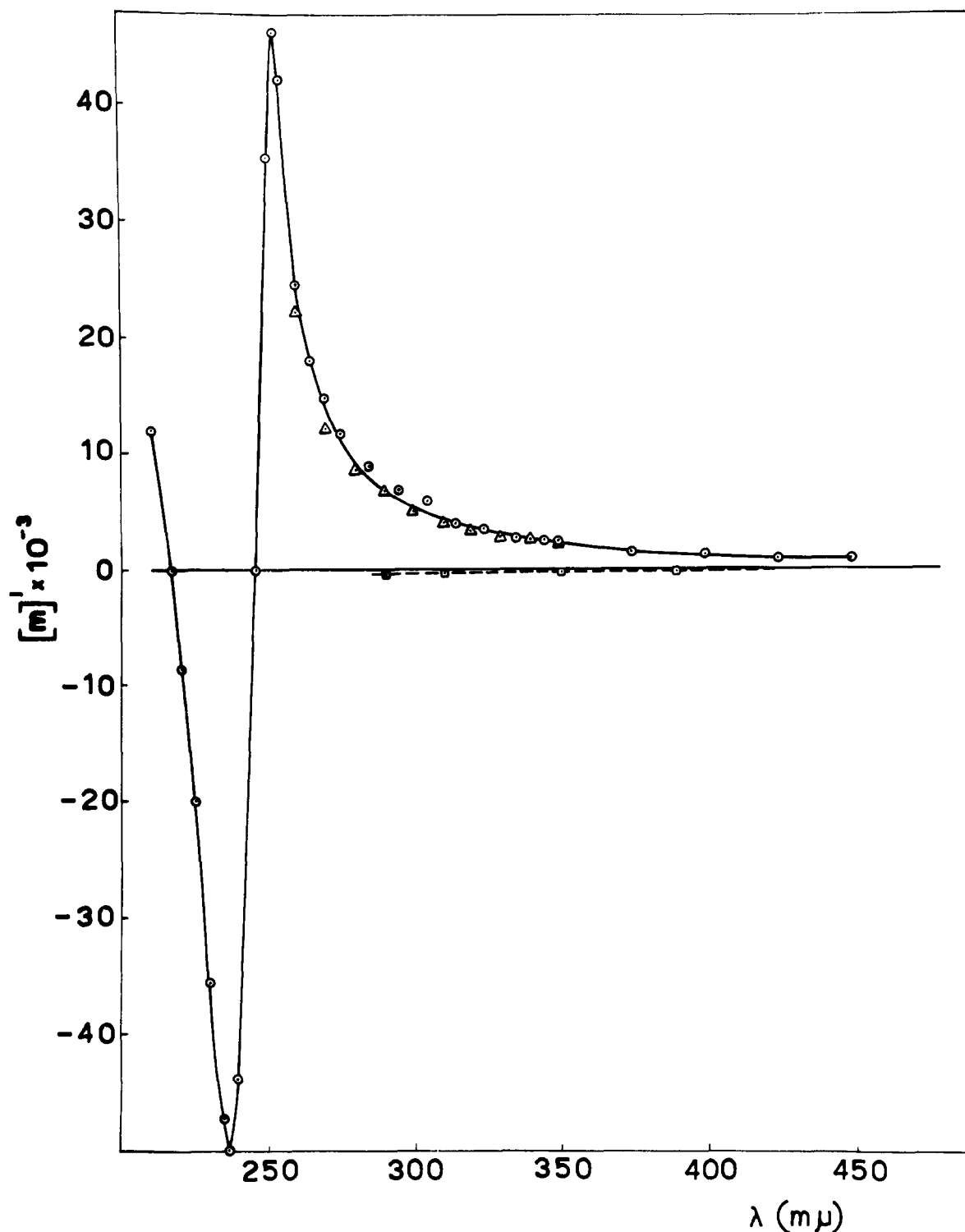
FIGURE 1: Optical rotatory dispersion of poly- N α -carbobenzoxy- L - p -aminophenylalanine in tetrahydrofuran (—) and in trifluoroacetic acid (---).
