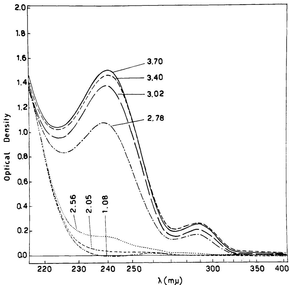
FIGURE 4: Ultraviolet absorption spectra of poly-L- p -aminophenylalanine as a function of pH in aqueous media. pH 1.08 (— · — · —), pH 2.05 (— — — —), pH 2.56 (· · · · ·), pH 2.78 (— · — · —), pH 3.02 (— — —), pH 3.40 (— · — · —), and pH 3.70 (————) as indicated.
