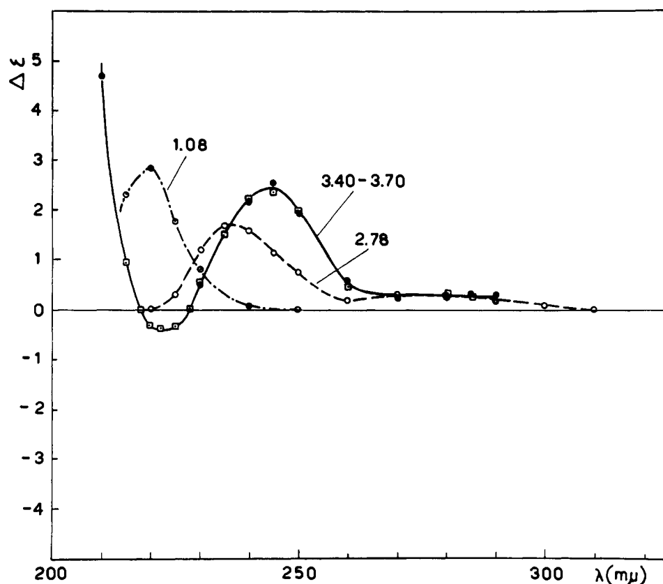
FIGURE 6: Circular dichroism of poly-L- p -aminophenylalanine as a function of pH in aqueous media. pH 1.08 (— · —), pH 2.78 (— · —), and pH 3.40–3.70 (—) as indicated.
