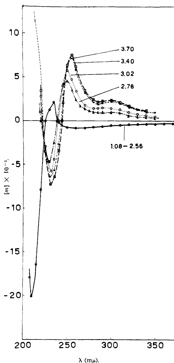
FIGURE 3: Optical rotatory dispersion of poly-L- p -aminophenylalanine as a function of pH in aqueous media. pH 1.08–2.56 (—), pH 2.78 (---), pH 3.02 (·····), pH 3.40 (----), and pH 3.70 (— · —) as indicated.
