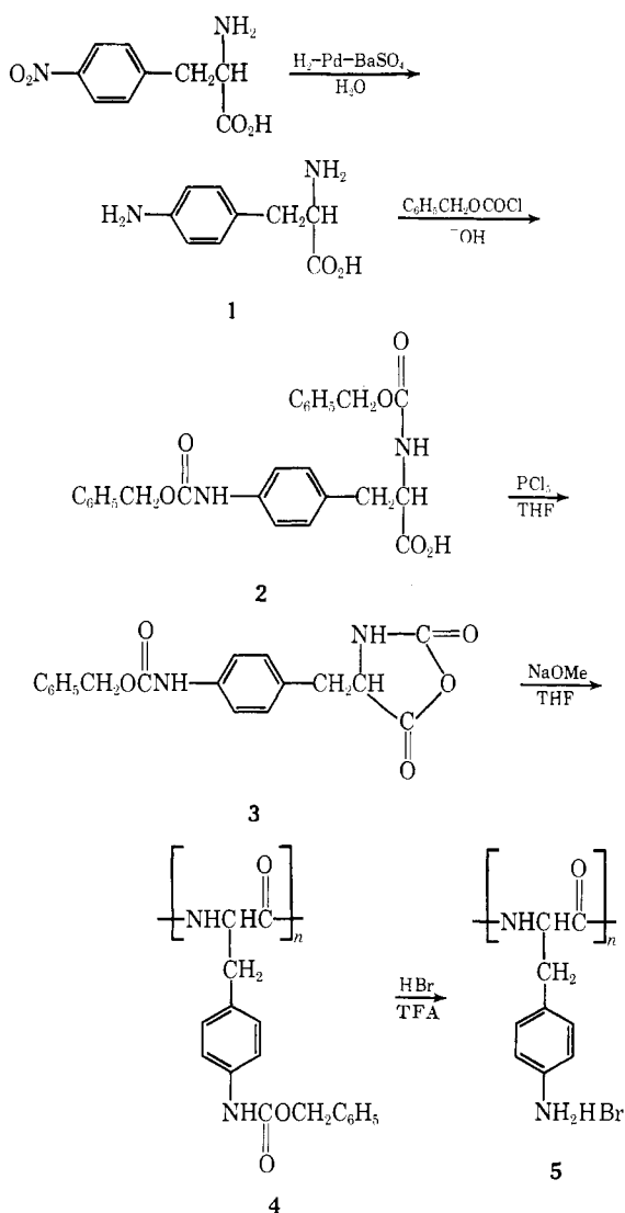
SCHEME I
