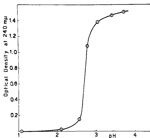
FIGURE 5: Optical density of poly-L- p -aminophenylalanine as a function of pH in aqueous media at 240 mμ. Concentration is 0.1%. The cell path is 0.5 mm.
